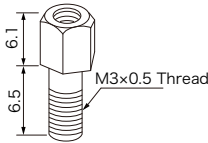
Jack Socket (17L-003 □ 1)
