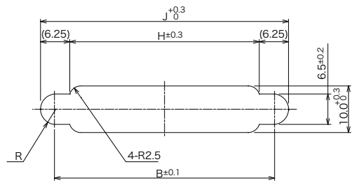
Panel Mounting Dimensions(Rear Mounting)
