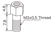
Jack Socket (17L-003 □ 3)
