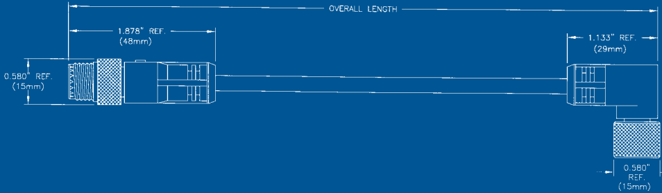
STRAIGHT TO 90° DOUBLE ENDED MALE / FEMALE
