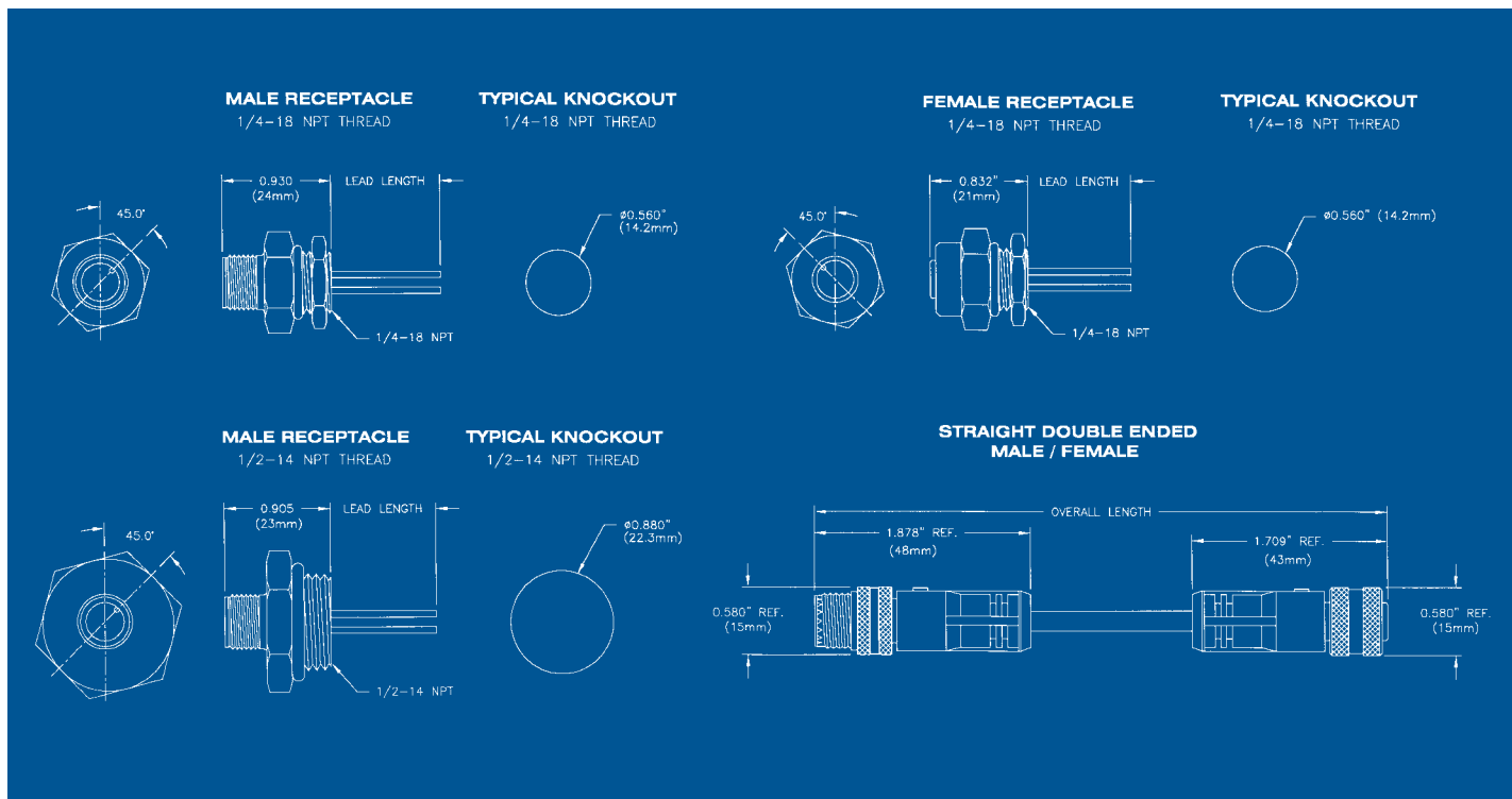
Anti-vibration coupling nuts standard.
