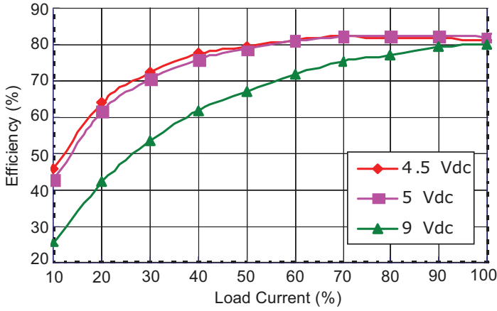
PDQ2-D5-D15-S Efficiency Curve (Efficiency vs. Line Voltage and Load Current)
