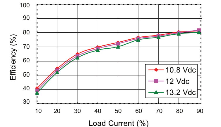
PCN1-S12-D15-M Efficiency Curve (Efficiency vs. Line Voltage and Load Current)
