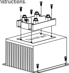
fig. 1 DP Series SSC mounted on HS053 heat sink (A)
