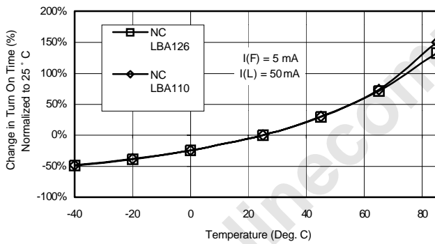
L. On Time vs. Ambient Temperature
