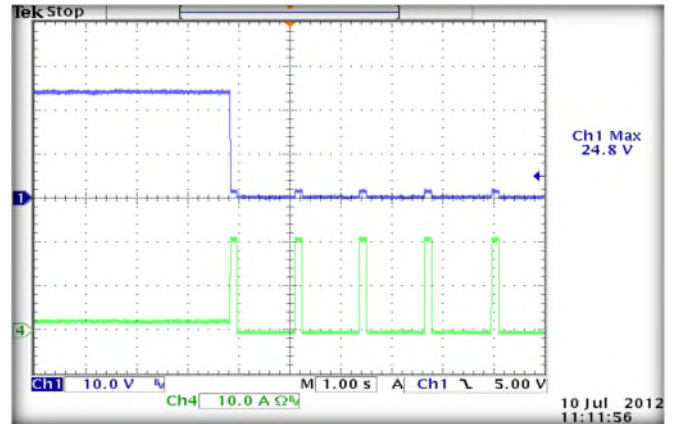
24V OUT, 264VAC
