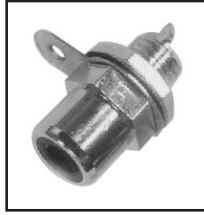
30-425-Bk Black 30-425-RD Red RCA-type mini Audio Jack with hex nut grip, hex nut and solder lug. Single hole mount. 1/4" hole. 9mm hex base. Bushing length .27".
