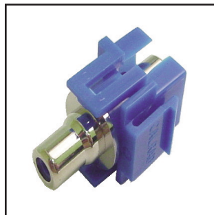
RGB+VIDEO RCA KEYSTONE INSERT RCA Female to Female jacks with colored inserts of Blue, Green, Ivory, Red, White or Yellow, Nickel plated. Specify color when ordering. 72-300-BK ..... Black 72-300-BU ..... Blue 72-300-GN ..... Green 72-300-IV ..... Ivory 72-300-OR ..... Orange 72-300-RD ..... Red 72-300-WH ..... White 72-300-YL ..... Yellow Gold Version available example order as " 72-300G-COLOR
