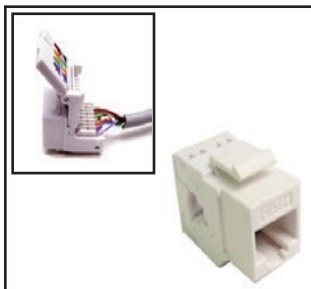
UL 1GHz RJ45 BROADBAND CAT 6 TOOLLESS, KEYSTONE JACK Secure self-terminating IDC mechanism allows for tool free installation. Gold plated 50 microns 72-401-WH .....White
