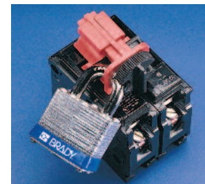
Universal Multi-Pole Lockout works with most two or three pole breakers utilizing a tie-bar.
