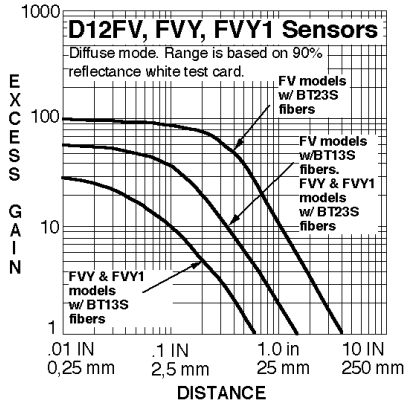
Diffuse Mode
