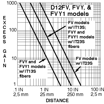
Opposed Mode
