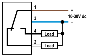
PNP (Sourcing) Standard Wiring
