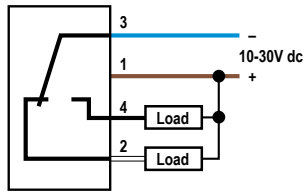
NPN (Sinking) Standard Wiring
