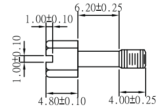
UNC #4-40 Hexscrew
