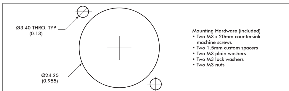
MOUNTING CUT-OUT DIMENSIONS
