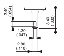
Quick-connect Z1
