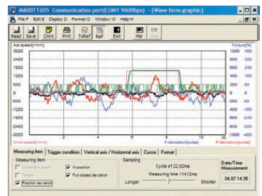
Graphic waveform display
