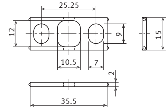
External dimensions
