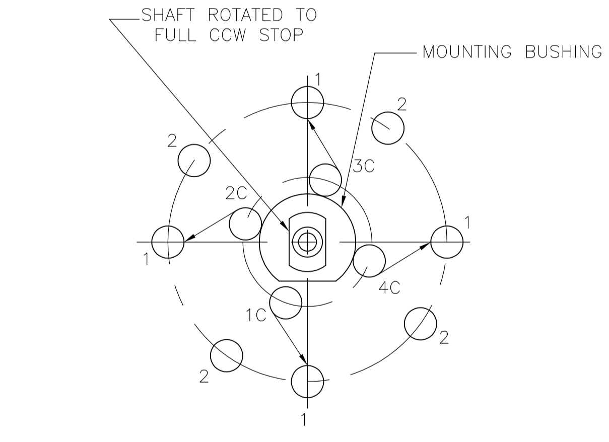
DIAGRAM LOOKING AT SHAFT END
