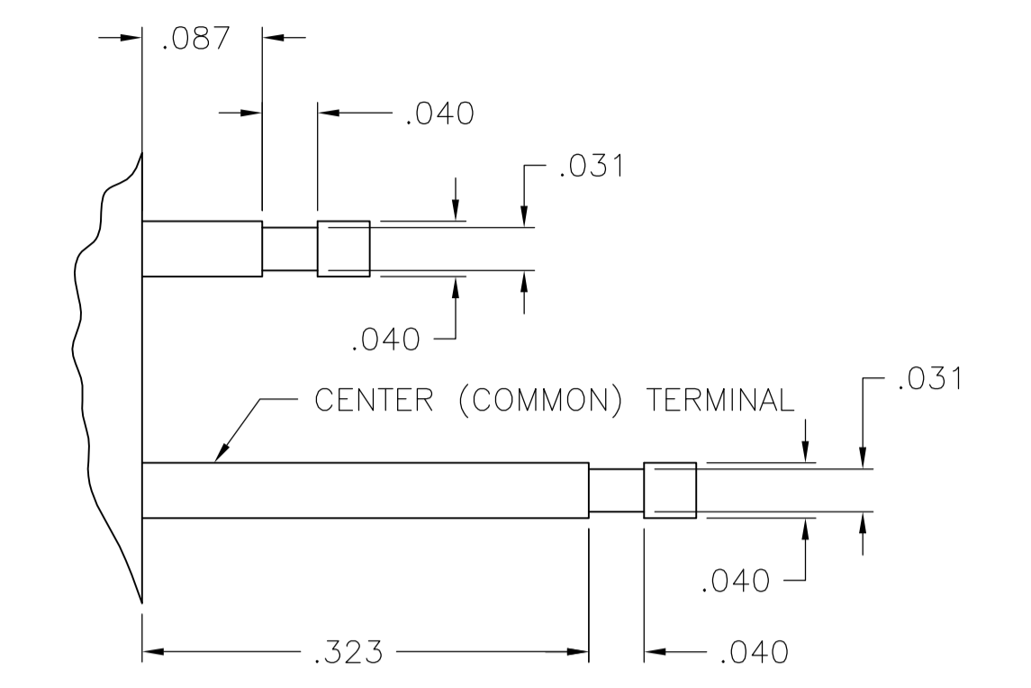
TYPICAL TERMINAL DETAIL
