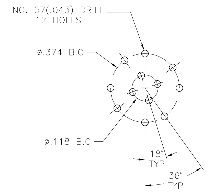
P.C MOUNTING DIMENSIONS
