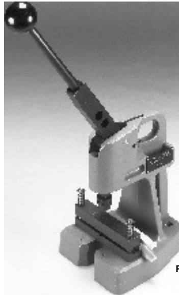
Manual Miniature Application Frame Assembly 91295-1 with Cover Closing Kit 543518-1
