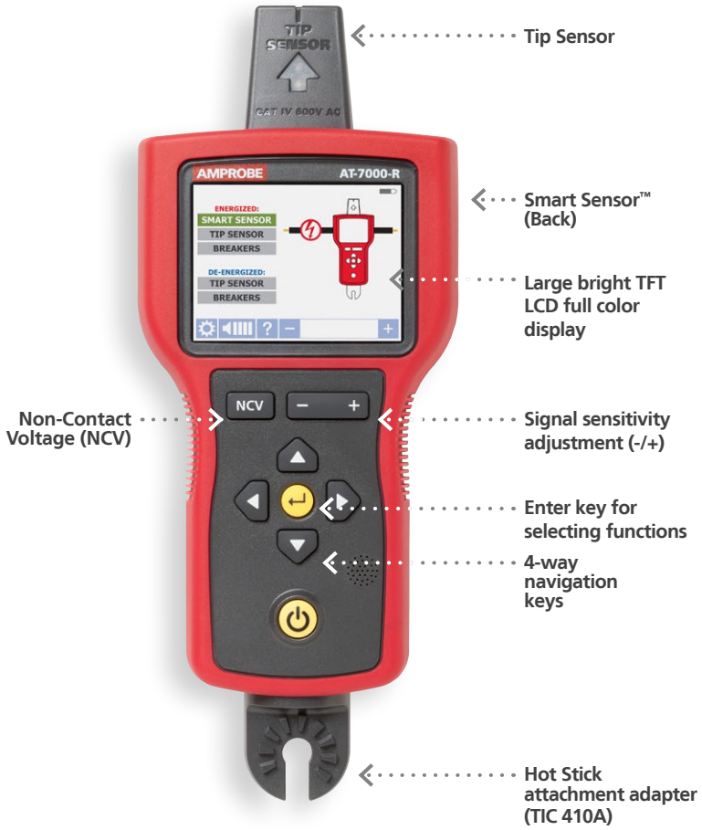
AT-7000-R Receiver
