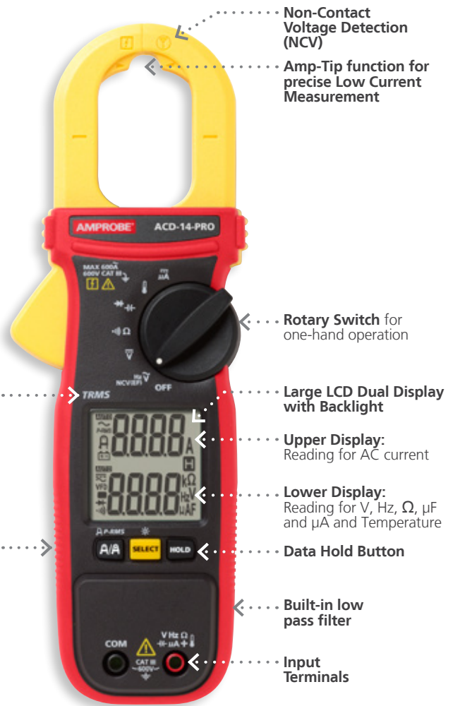
ACD-14-PRO Dual Display 600 A TRMS Clamp Multimeter
