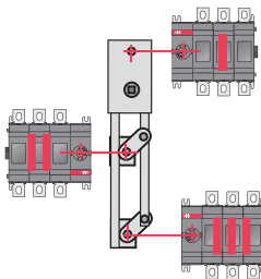
Change-over and by-pass switches
