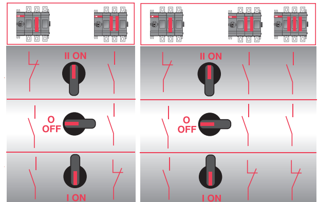
Change-over switches
