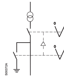
Mechanical interlock
