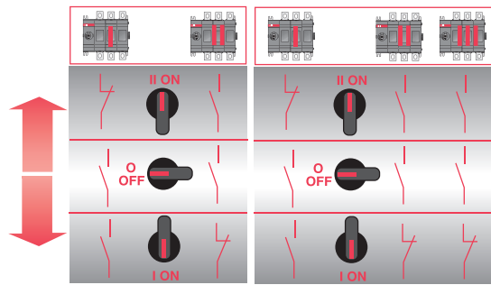
Change-over switches By-pass switches
