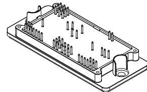
Q2PACK NEGATIVE SOLDER PINS CASE 180BM
