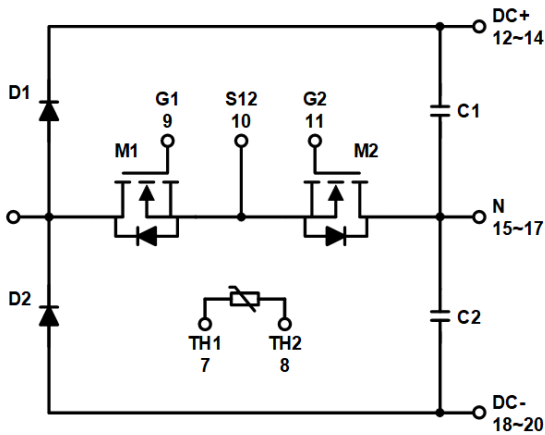
Figure 1. NXH020U90MNF2 Schematic Diagram
