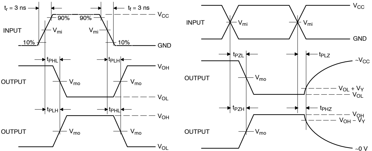
Figure 6. Switching Waveforms
