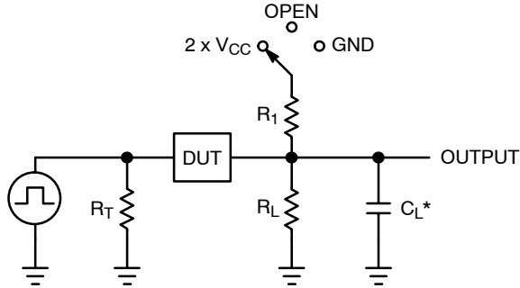
Figure 5. Test Circuit
