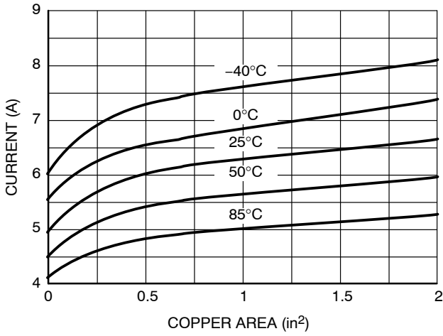
Figure 15. Thermal Limit vs. Copper Area and Ambient Temperature
