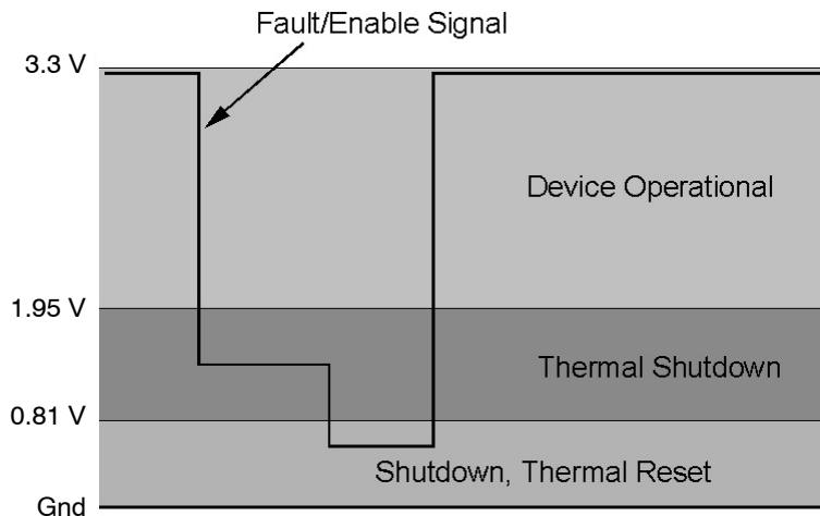
Figure 22. Fault/Enable Signal Levels
