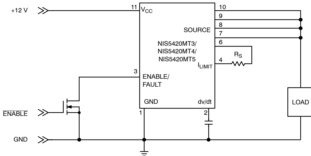
Figure 5. Application Circuit with Kelvin Current Sensing
