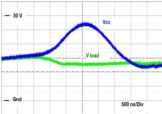
Figure 13. Input Transient Response
