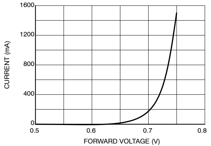
Figure 14. Body Diode Forward Characteristics
