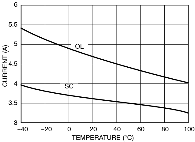
Figure 19. Kelvin Current Sensing Levels vs. Temperature for 15 \Omega Sense Resistor
