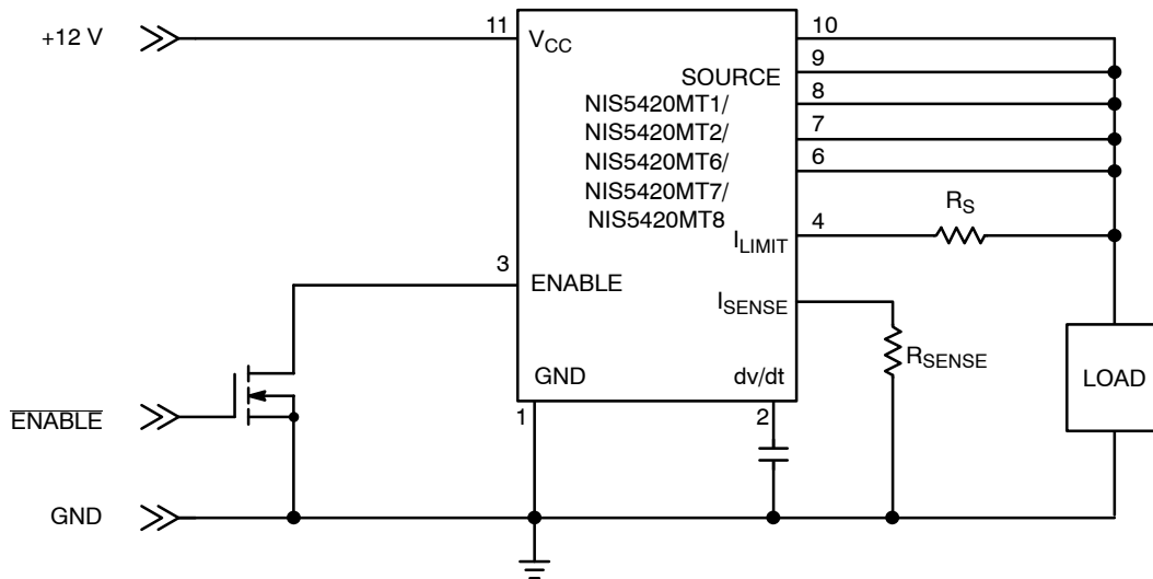
Figure 6. Application Circuit with Direct Current Sensing (NIS5424 only)
