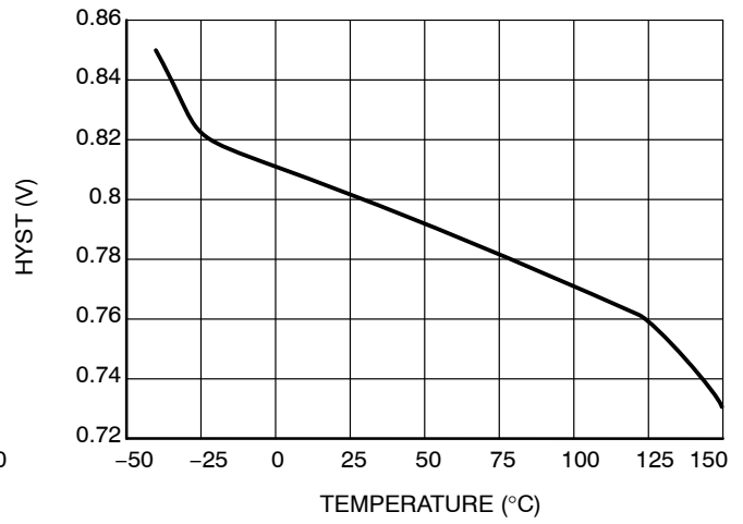
Figure 10. UVLO Hysteresis
