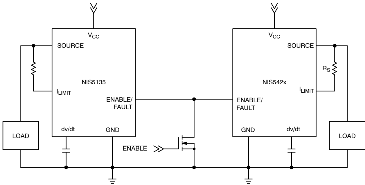
Figure 8. Common Thermal Shutdown
