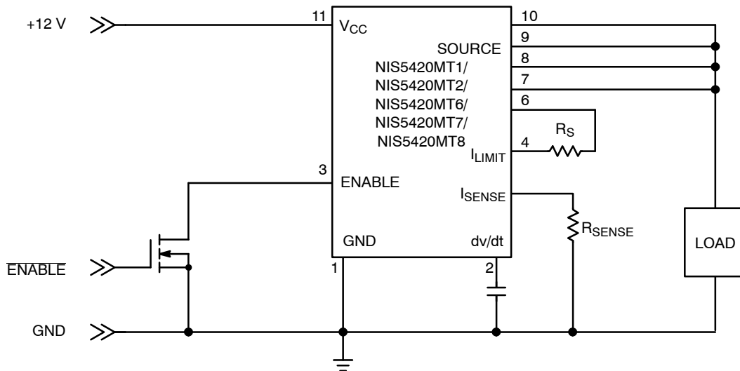
Figure 7. Application Circuit with Kelvin Current Sensing (NIS5424 only)
