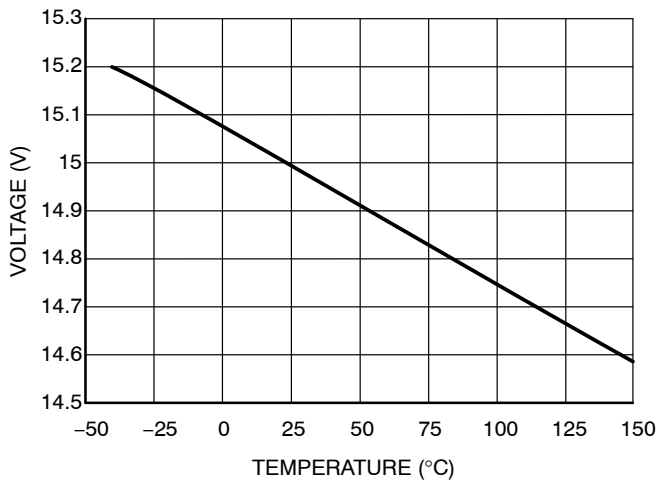
Figure 11. Output Clamping Voltage
