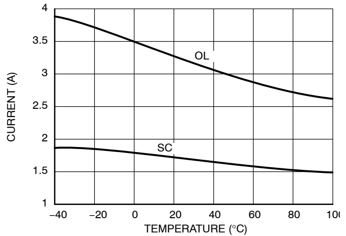
Figure 20. Kelvin Current Sensing Levels vs. Temperature for 33 \Omega Sense Resistor
