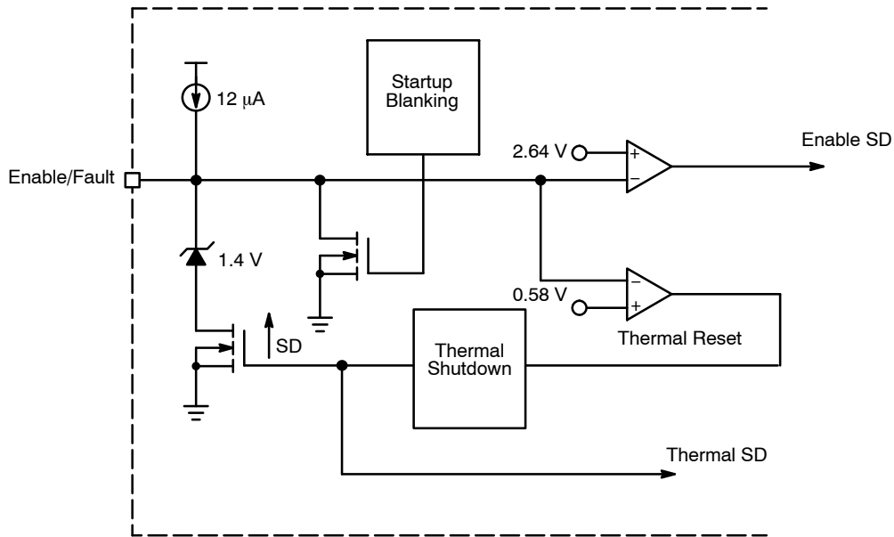
Figure 23. Enable/Fault Simplified Circuit
