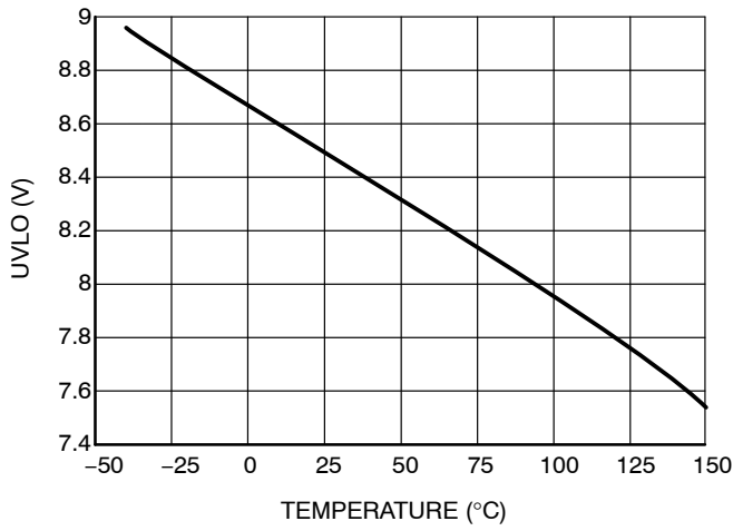
Figure 9. UVLO Turn-On
