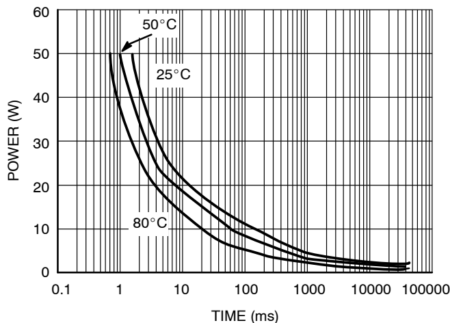
Figure 3. Power Dissipation vs. Thermal Trip Time
