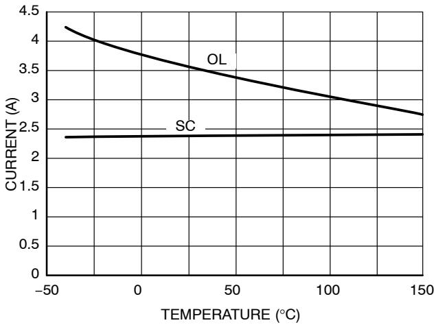
Figure 17. Direct Current Sensing Levels vs. Temperature for 27 \Omega Sense Resistor
