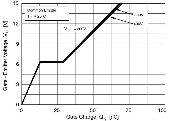
Figure 8. Gate Charge
