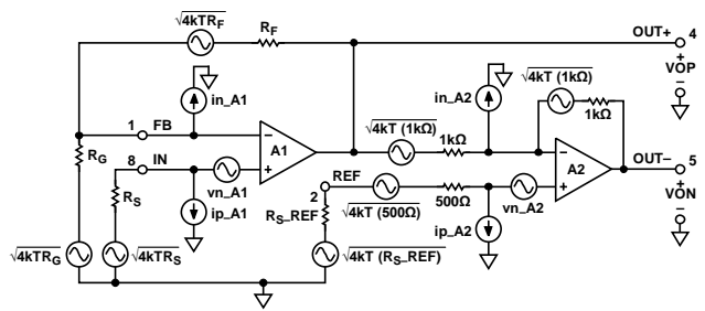
Figure 52. Noise Sources
